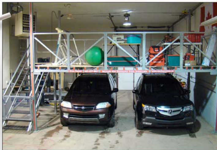
Mechano Max structure erected in just 2 days. Room for cars again in the two car garage.
